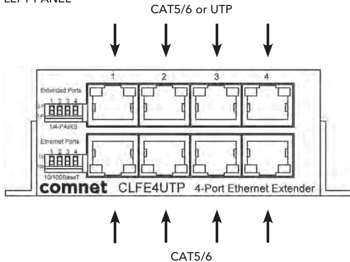
FIGURE 3 - CLFE4UTP
