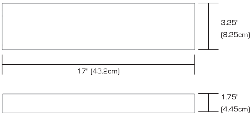
Dimensions are for the CLFE8UTP and CLFE16UTP ComNet modules
