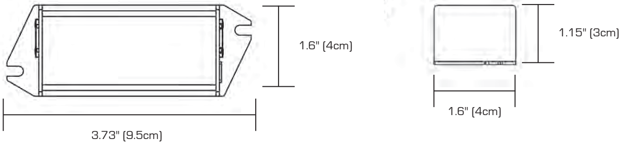
Dimensions are for the CLFE1UTP standalone ComNet module
