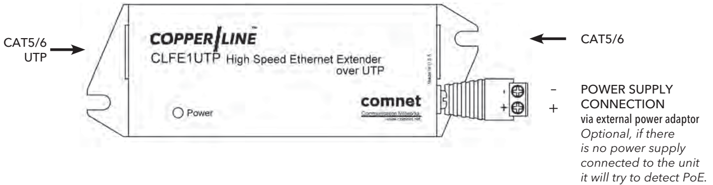
FIGURE 2 - CLFE1UTP
