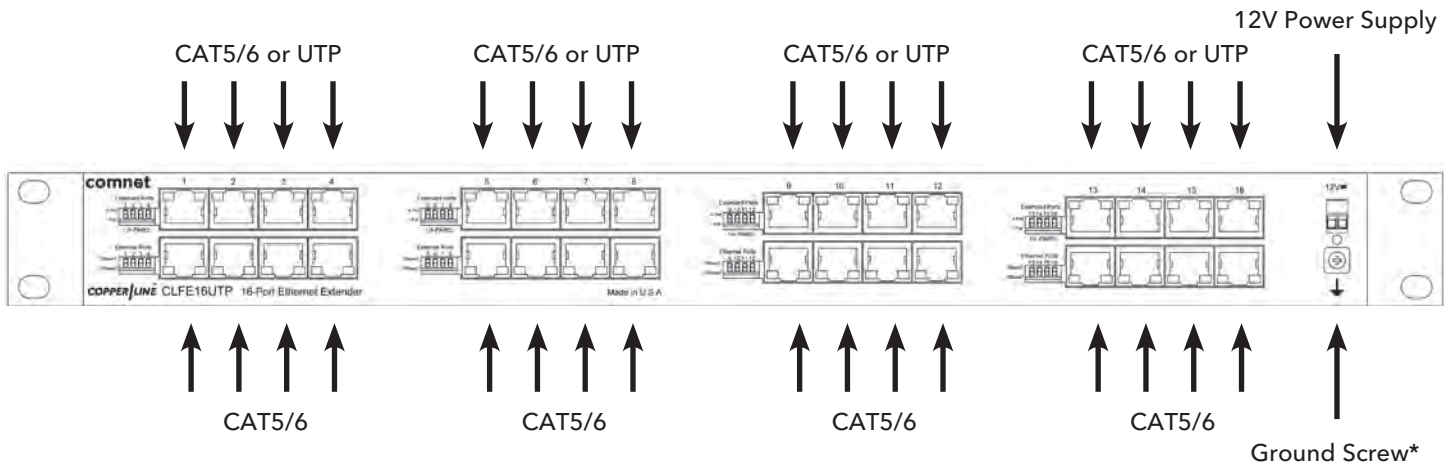
FIGURE 5 - CLFE16UTP
