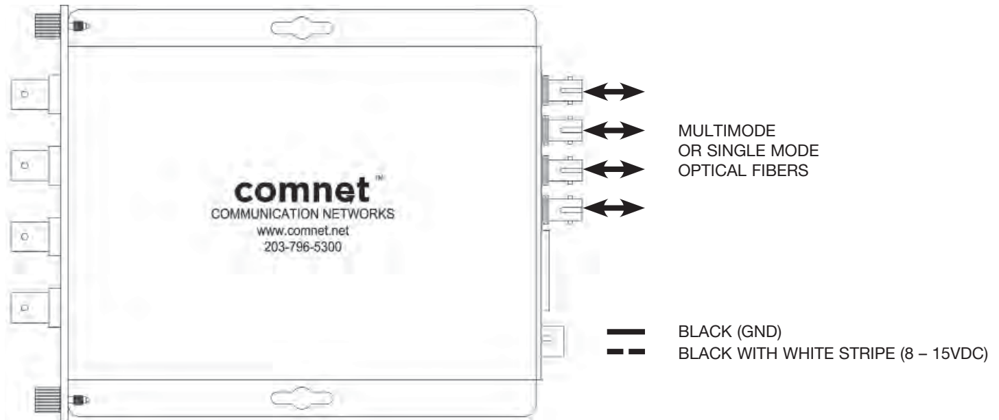
FIGURE 1 – FVR4C4B4 RECEIVER
