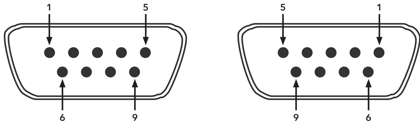
DB-9 Male DB-9 Female
