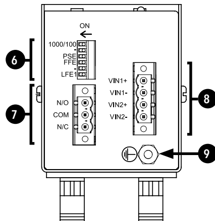
Figure 2 - RLMCSFP24DC and RLMCSFP48DC Bottom Panel
