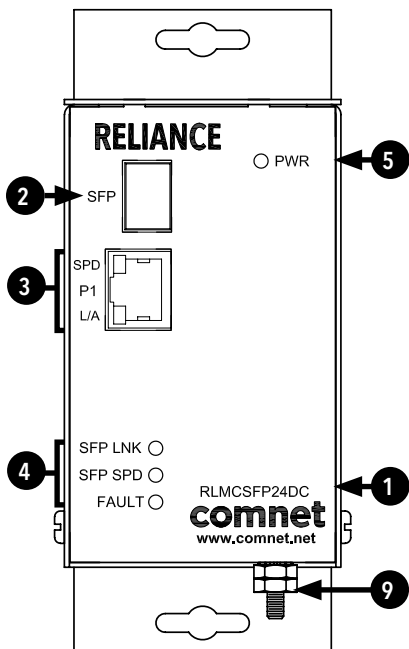
Figure 1 - RLMCSFP Series Front Panel
