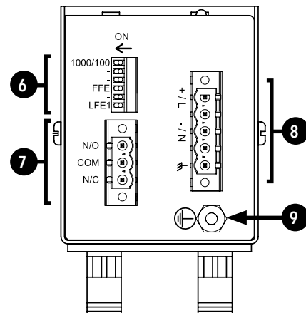
Figure 3 - RLMCSFPHV Bottom Panel
