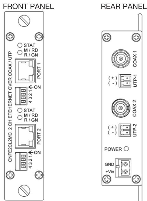
FIGURE 2 – CNFE2CL2MC STANDARD SIZE UNIT
