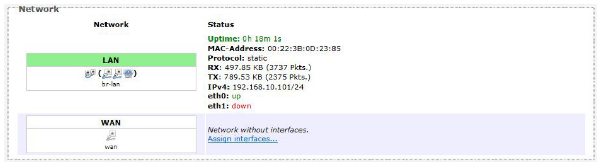
Figure 10: Network summary.
