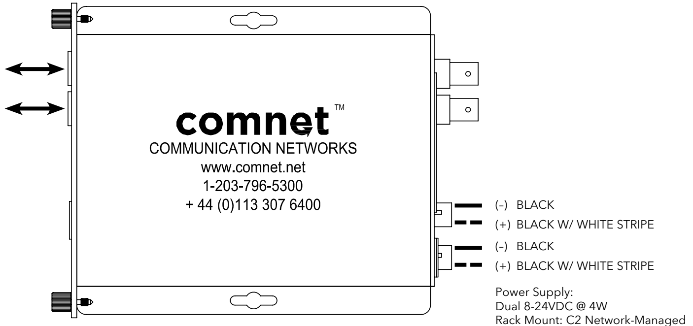
FIGURE 1 - FVT/FVR20D211C4E TRANSMITTER AND RECEIVER
