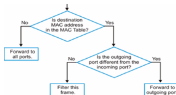
Figure: MAC Table Flowchart
