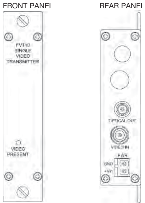
FIGURE 2 – FVT10 TRANSMITTER
