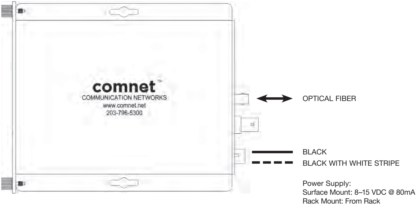
FIGURE 1 – FVT10 TRANSMITTER
