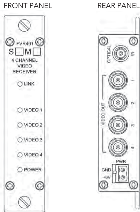
FIGURE 3 - FVR401 RECEIVER
