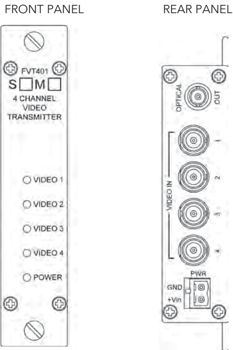
FIGURE 2 - FVT401 TRANSMITTER
