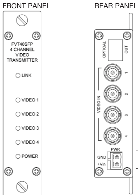
FIGURE 2 – FVT40SFP TRANSMITTER
