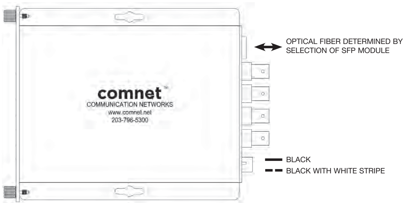
FIGURE 1 – FVT/FVR40SFP TRANSMITTER AND RECEIVER
