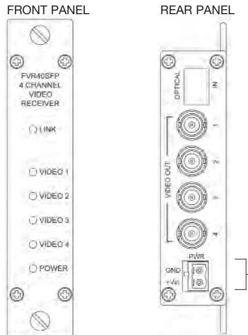
FIGURE 3 – FVR40SFP RECEIVER
