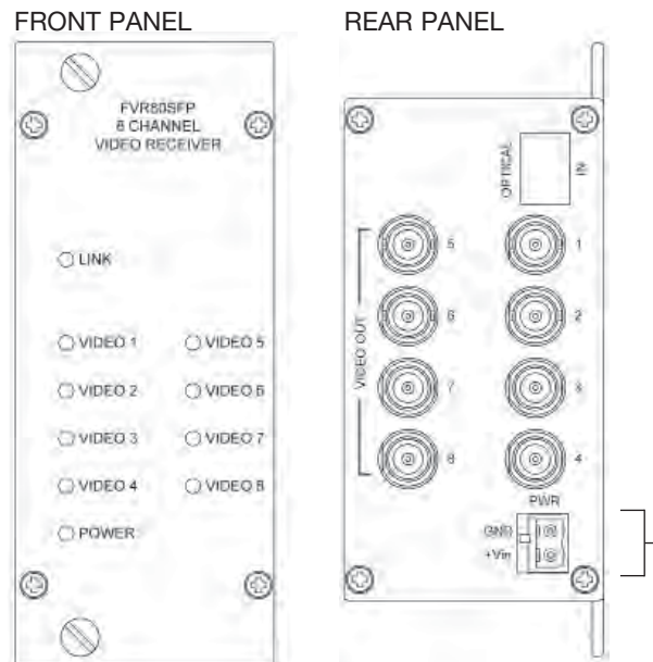
FIGURE 3 – FVR80SFP RECEIVER
