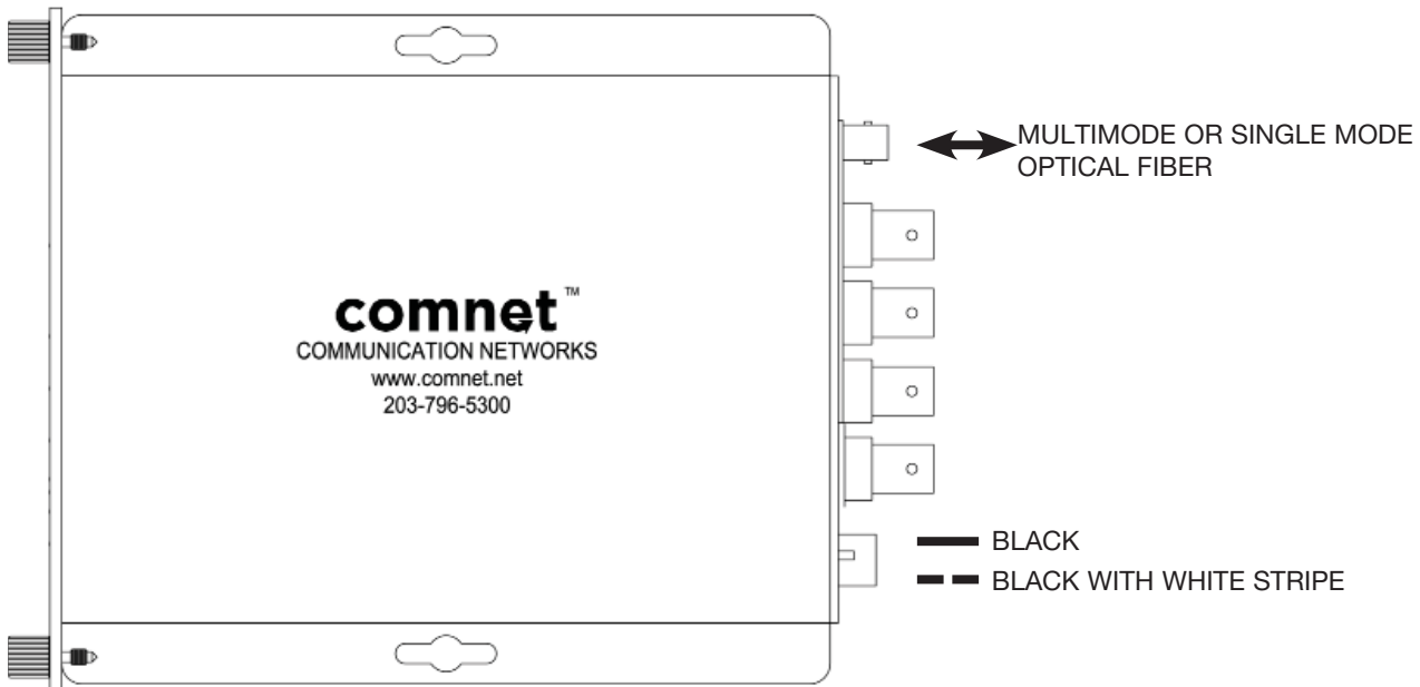
FIGURE 1 – FVT/FVR2014 TRANSMITTER AND RECEIVER
