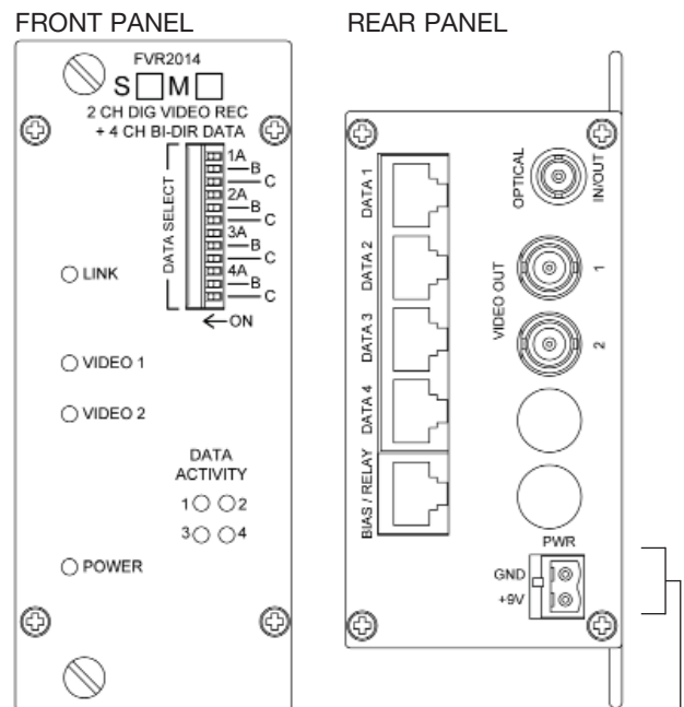
FIGURE 3 – FVR2014 RECEIVER
