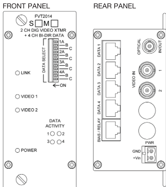
FIGURE 2 – FVT2014 TRANSMITTER
