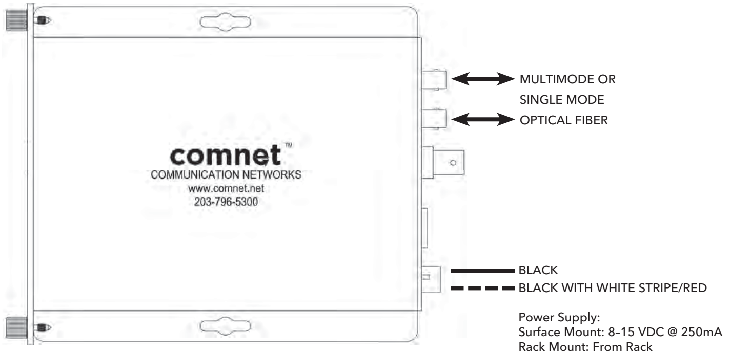
FIGURE 1 - FVT/FVR15M2
