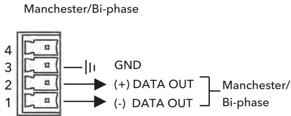
FIGURE 5 - DATA SETTINGS
