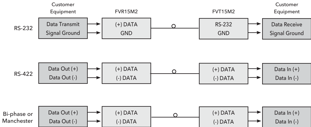
FIGURE 5 - DATA SETTINGS
