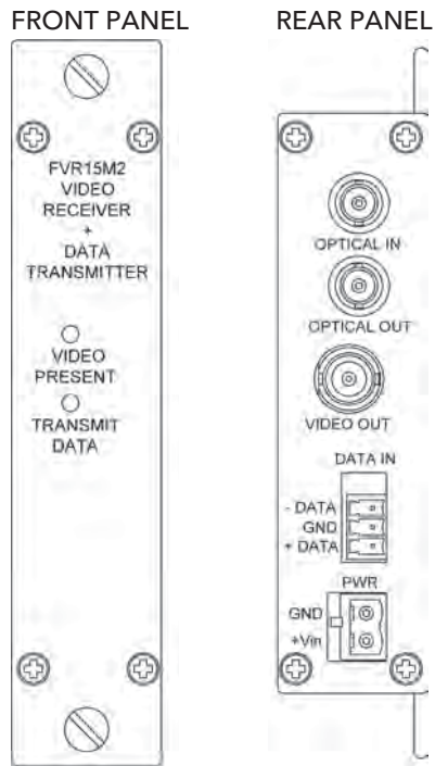
FIGURE 3 - FVR15M2 RECEIVER
