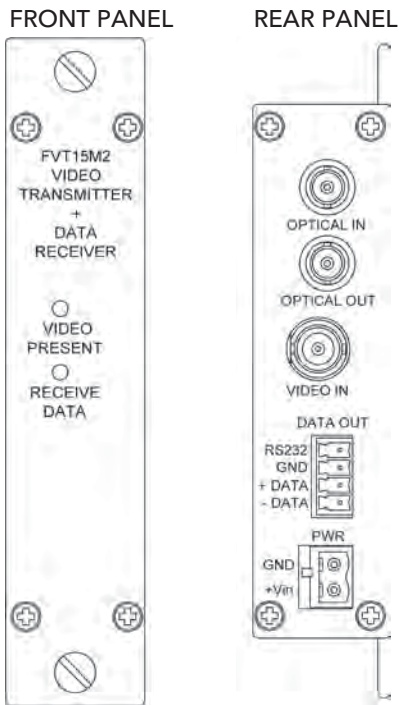
FIGURE 2 - FVT15M2 TRANSMITTER
