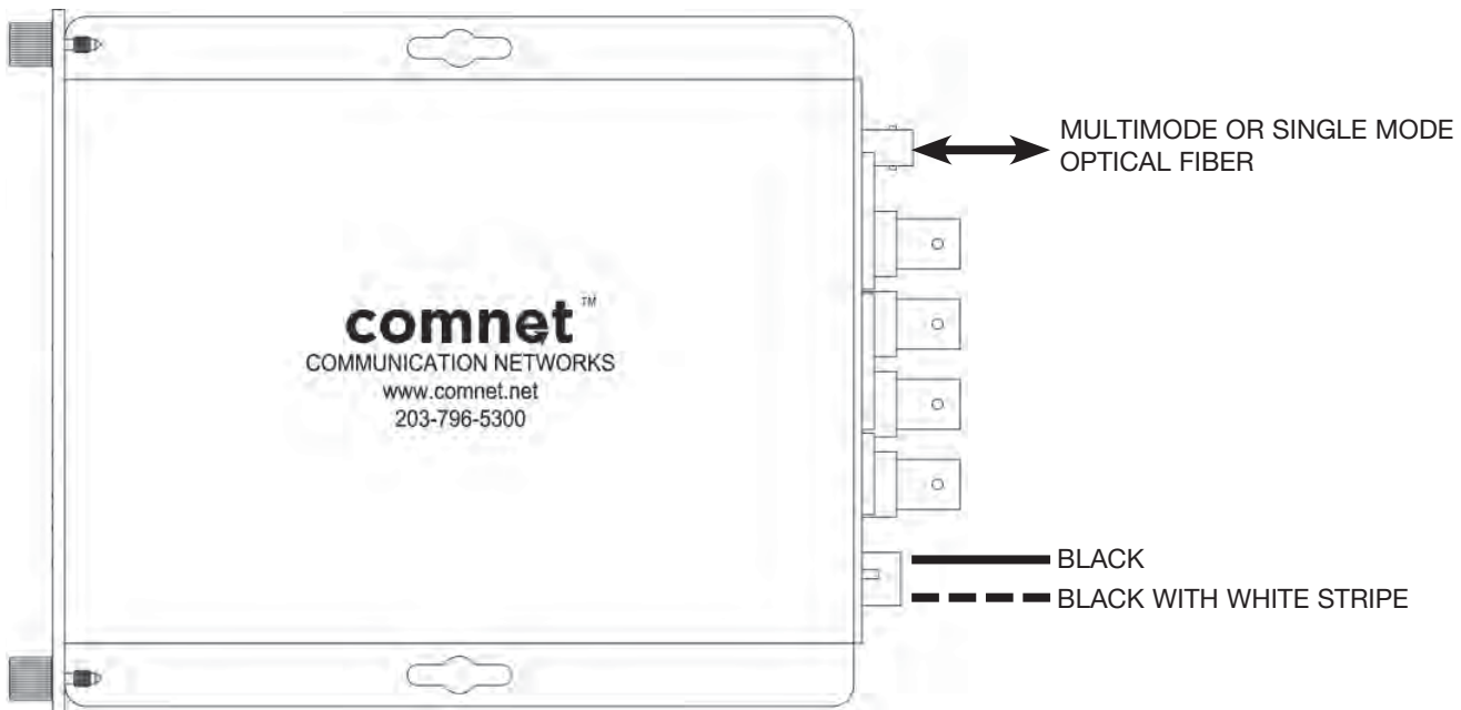
FIGURE 1 – FVT/FVR412 TRANSMITTER AND RECEIVER
