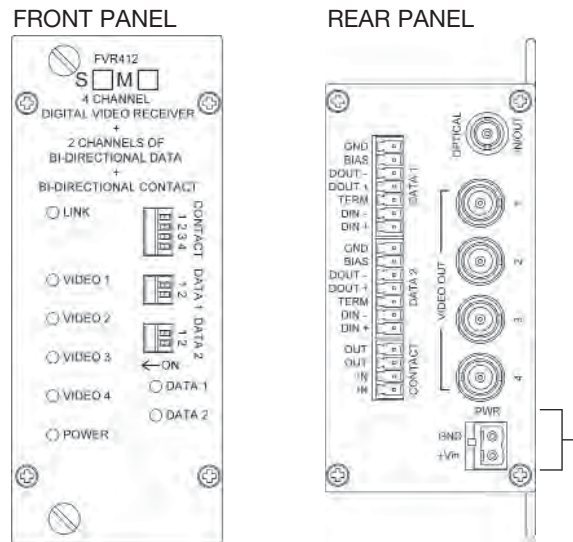
FIGURE 3 – FVR412 RECEIVER
