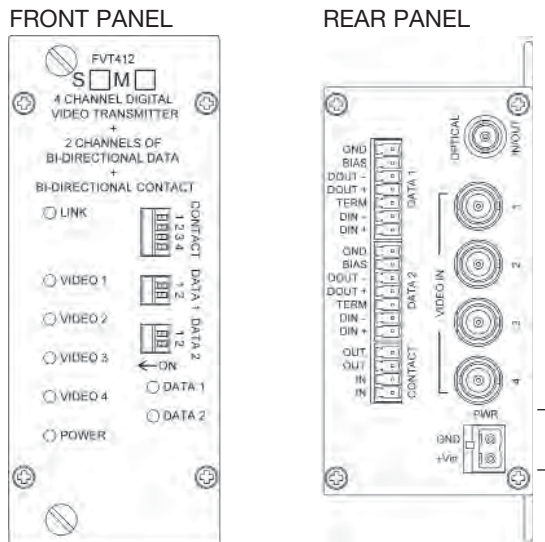
FIGURE 2 – FVT412 TRANSMITTER
