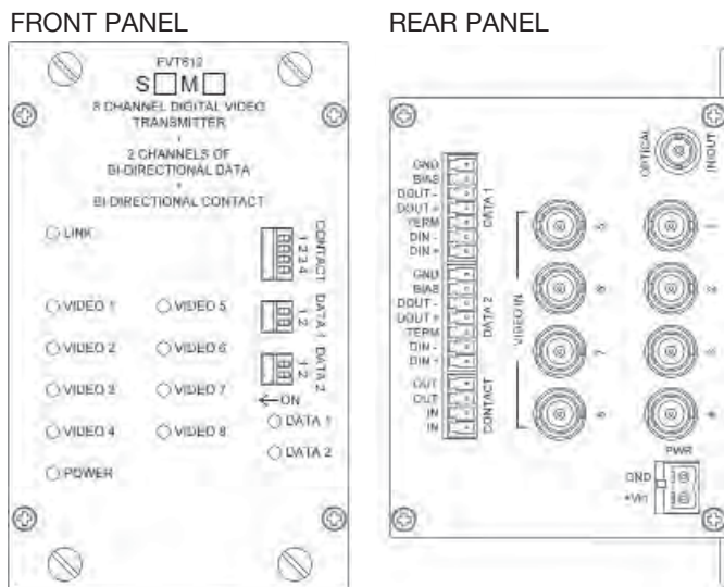
FIGURE 2 – FVT812 TRANSMITTER
