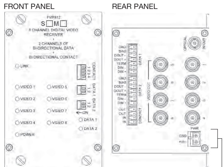
FIGURE 3 – FVR812 RECEIVER
