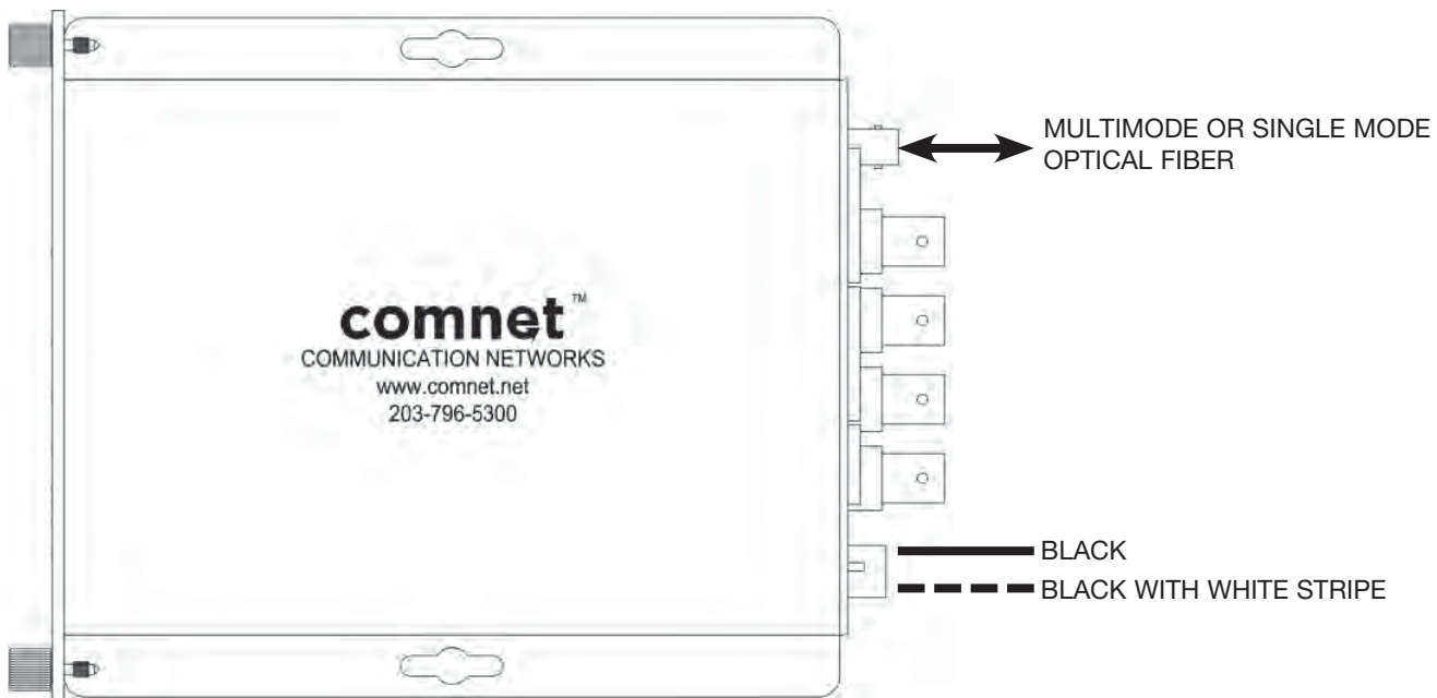
FIGURE 1 – FVT/FVR812 TRANSMITTER AND RECEIVER
