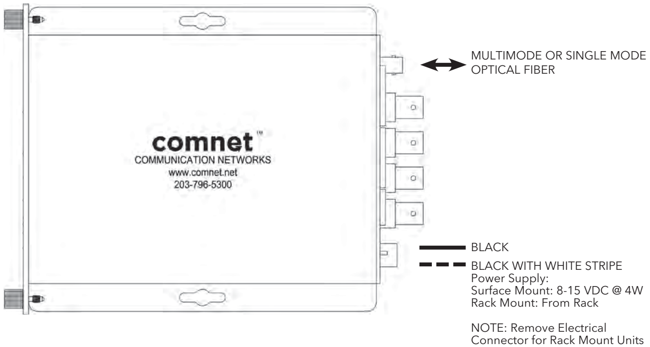
FIGURE 1 - FVT/FVR8012 TRANSMITTER AND RECEIVER
