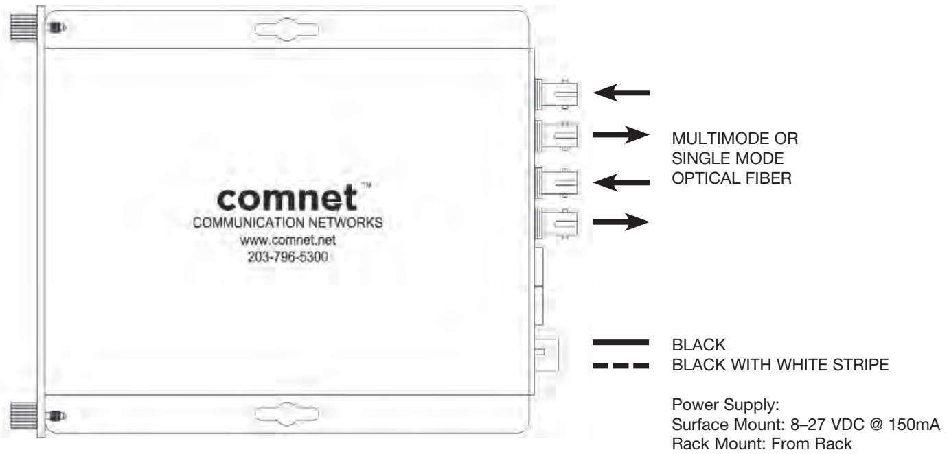
FIGURE 3 – FDC2 TRANSCEIVER
